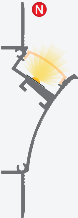
TIJUANA 34.8x98mm
