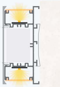
Pared / Wall: 8 modelos / models
