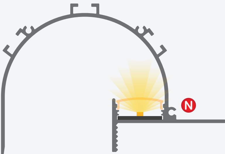
CARACAS 101x69mm
