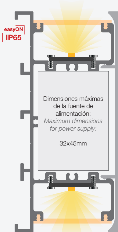
WASHINGTON 47x100mm
